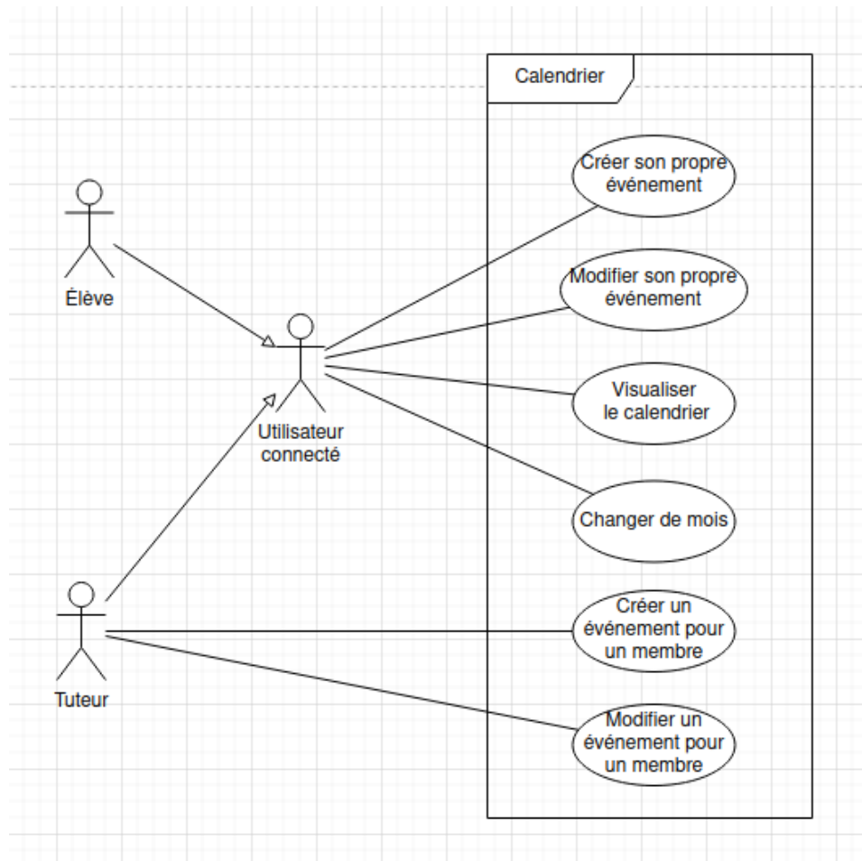
Use case Calendrier
