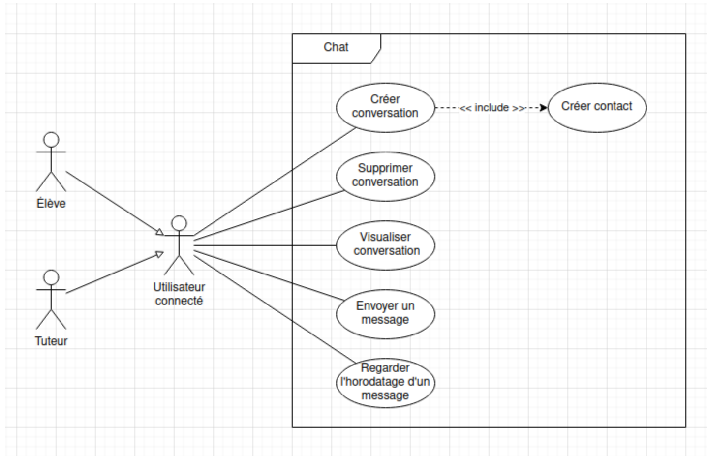
Use case Chat
