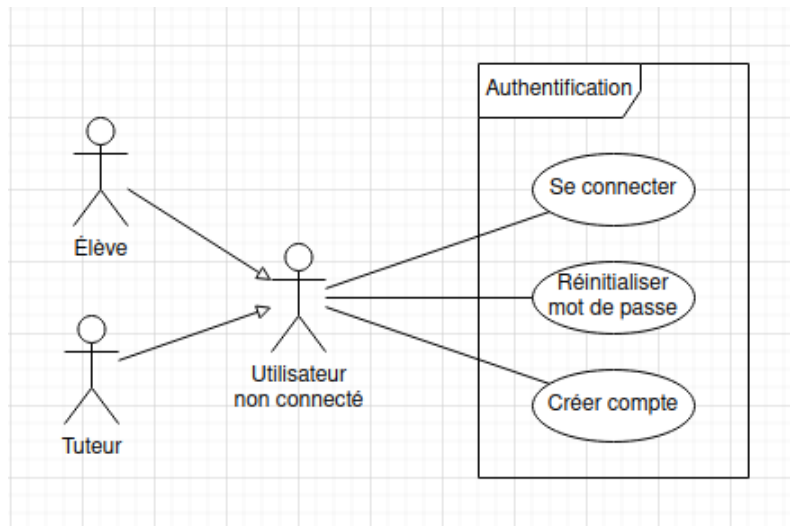
Use case authentication
